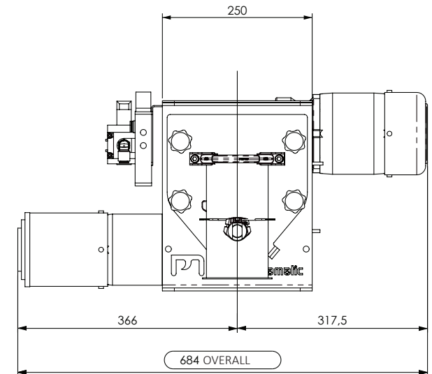
WITH FORCED VENTILATION FOR SCREW FEEDER ENGINE
